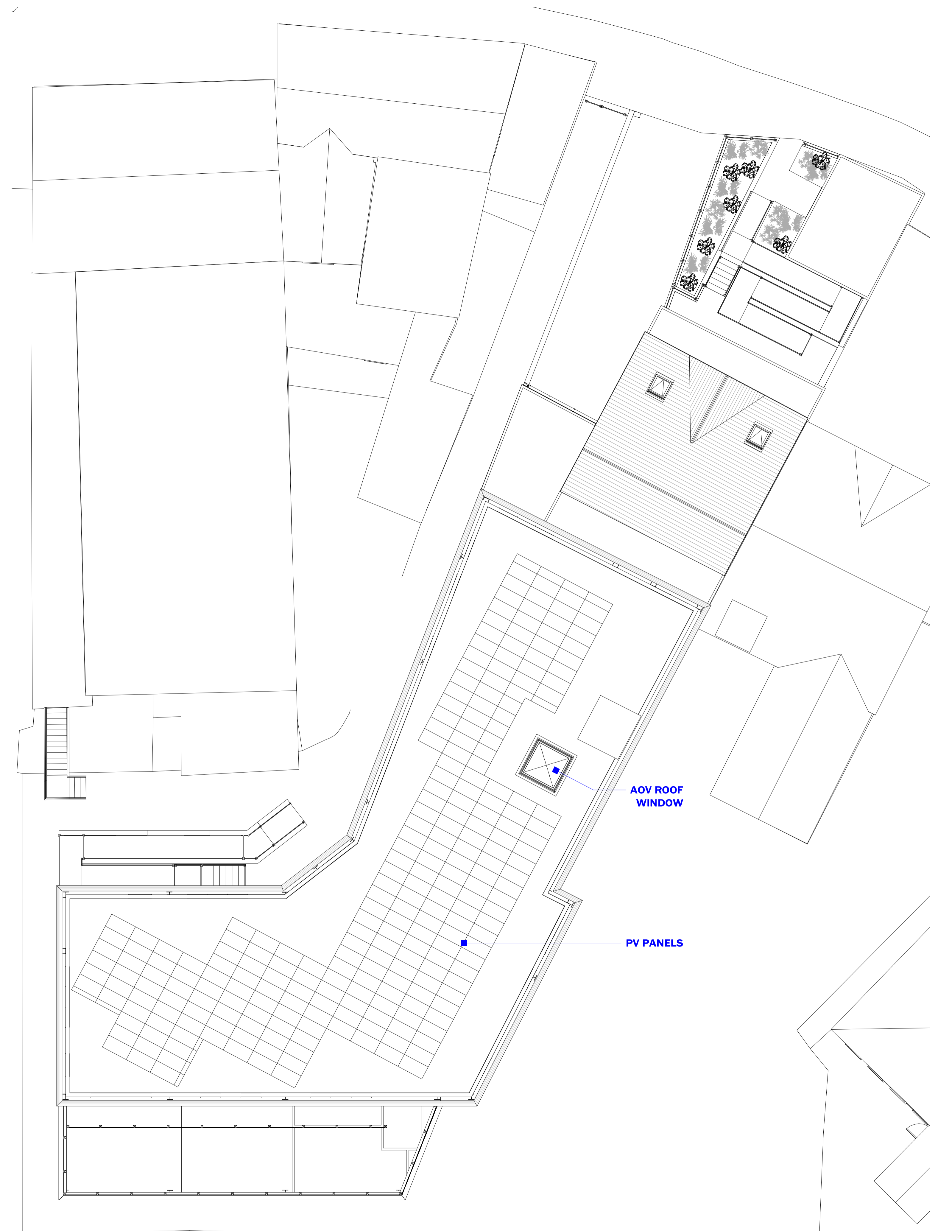
01 PROPOSED ROOF PLAN 1 : 100
