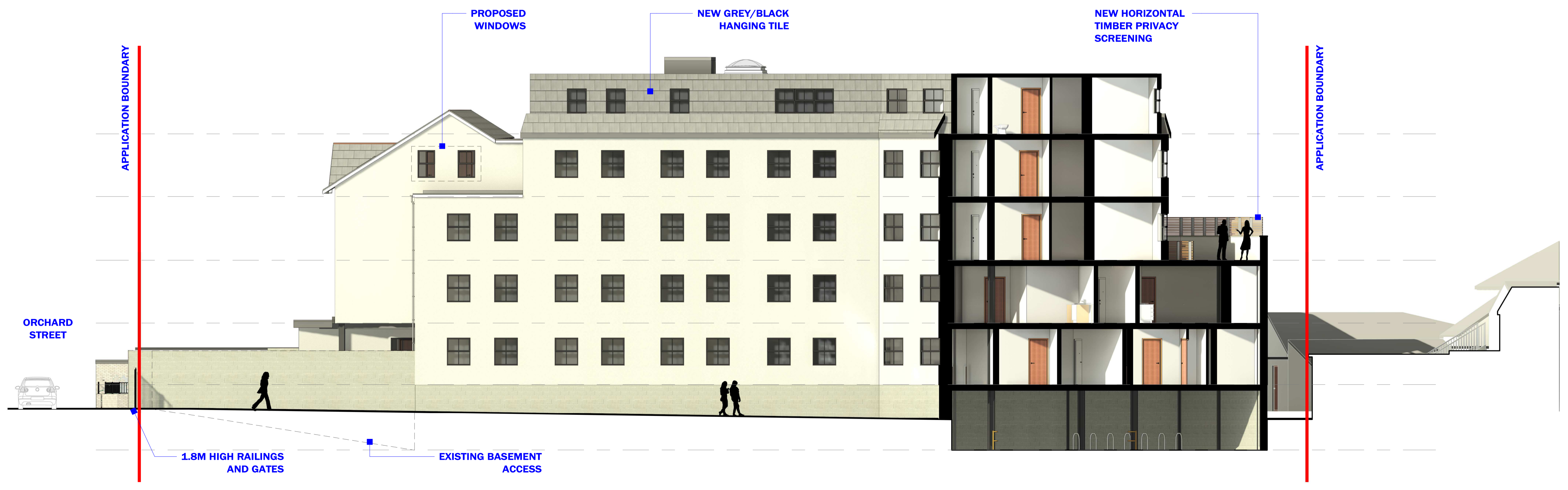
03 PROPOSED ELEVATION C 1:100
