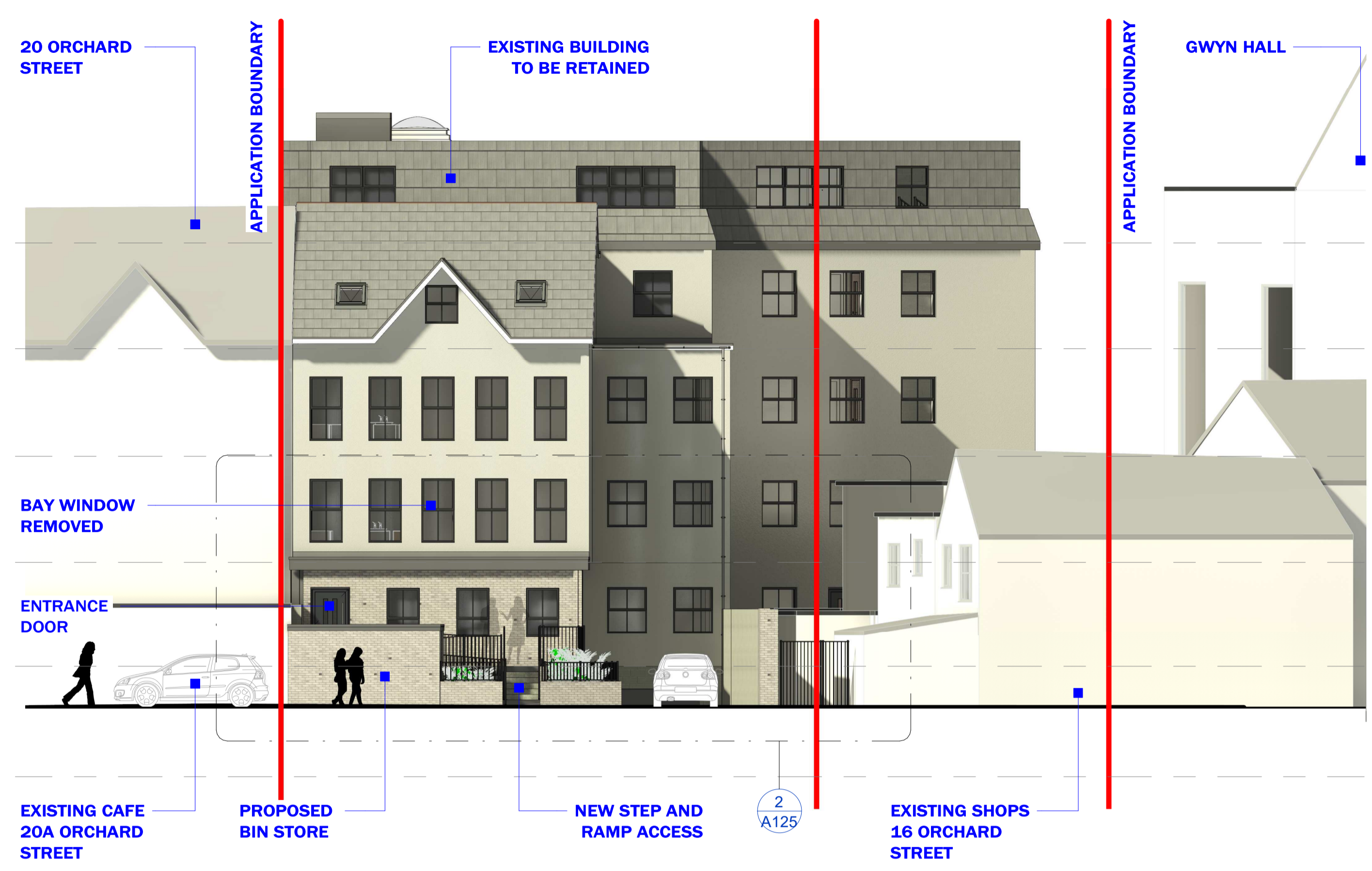
01 PROPOSED ELEVATION A 1:100
